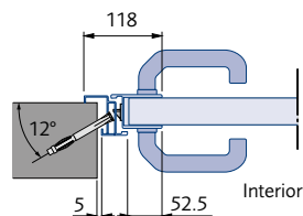
Profile 2: Opening outwards
