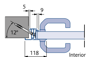
Profile 1: Only opening inwards
