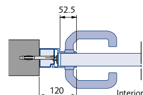
Profile 2: Opening inwards or outwards (inwards shown)
