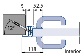
Profile 2: Opening inwards
