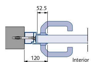
Profile 2: Opening inwards or outwards (inwards shown)
