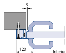
Profile 2: Opening inwards
