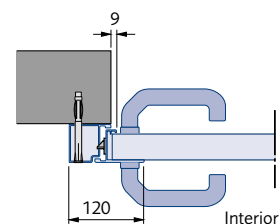
Profile 2: Opening inwards
