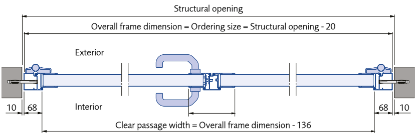
Profile 2: Only opening outwards
