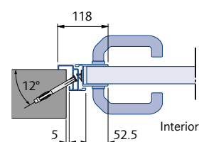
Profile 1: Only opening inwards
