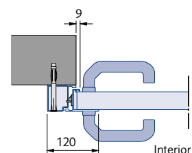
Profile 2: Opening inwards or outwards (inwards shown)
