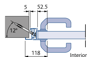
Profile 2: Opening inwards
