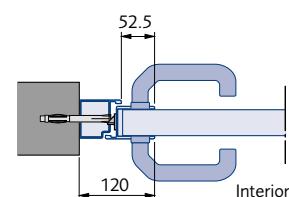
Profile 2: Opening inwards
